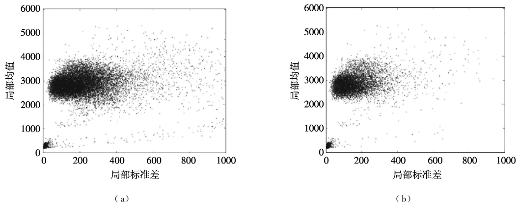
图 5 AVIRIS 辐射图像(图 1(b))第 67 波段含边缘块剔出前后局部均值与局部标准差散点图 Fig 5 Two scatter plots of local means versus local standard deviations from band 67 of AVIRIS radiance images (Figure 1 (b)) before and after blocks containing edges are removed
