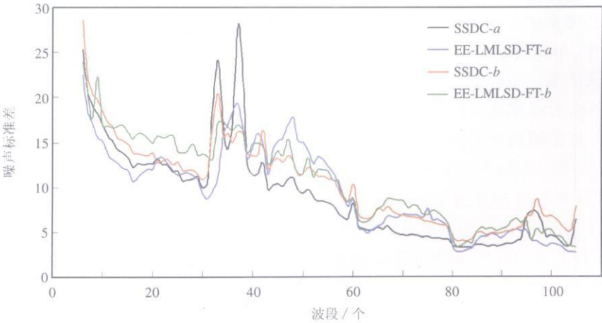
(C)1994-2021 China Academic Journal Electronic Publishing House. All rights reserved. http://www.cnki.net 图 10 同时利用两种操作方法对图 1 中 AVIRIS 辐射图像进行噪声评估的结果 Fig 10 Estimations of the noise for AVIRIS radiance images shown in Figure 1 via the both methods at the same time
